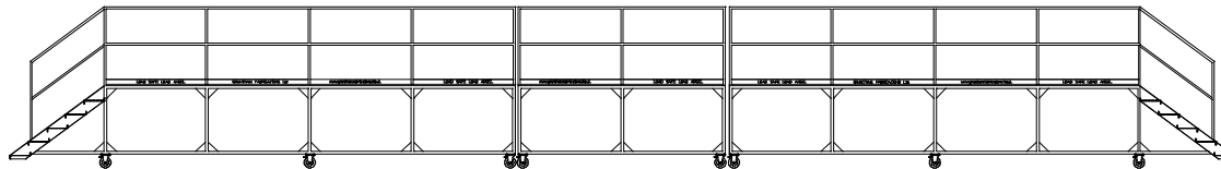
Left and Right Hand 6 Meter Platforms plus one 3 Meter module makes 15 meter single side Platform
